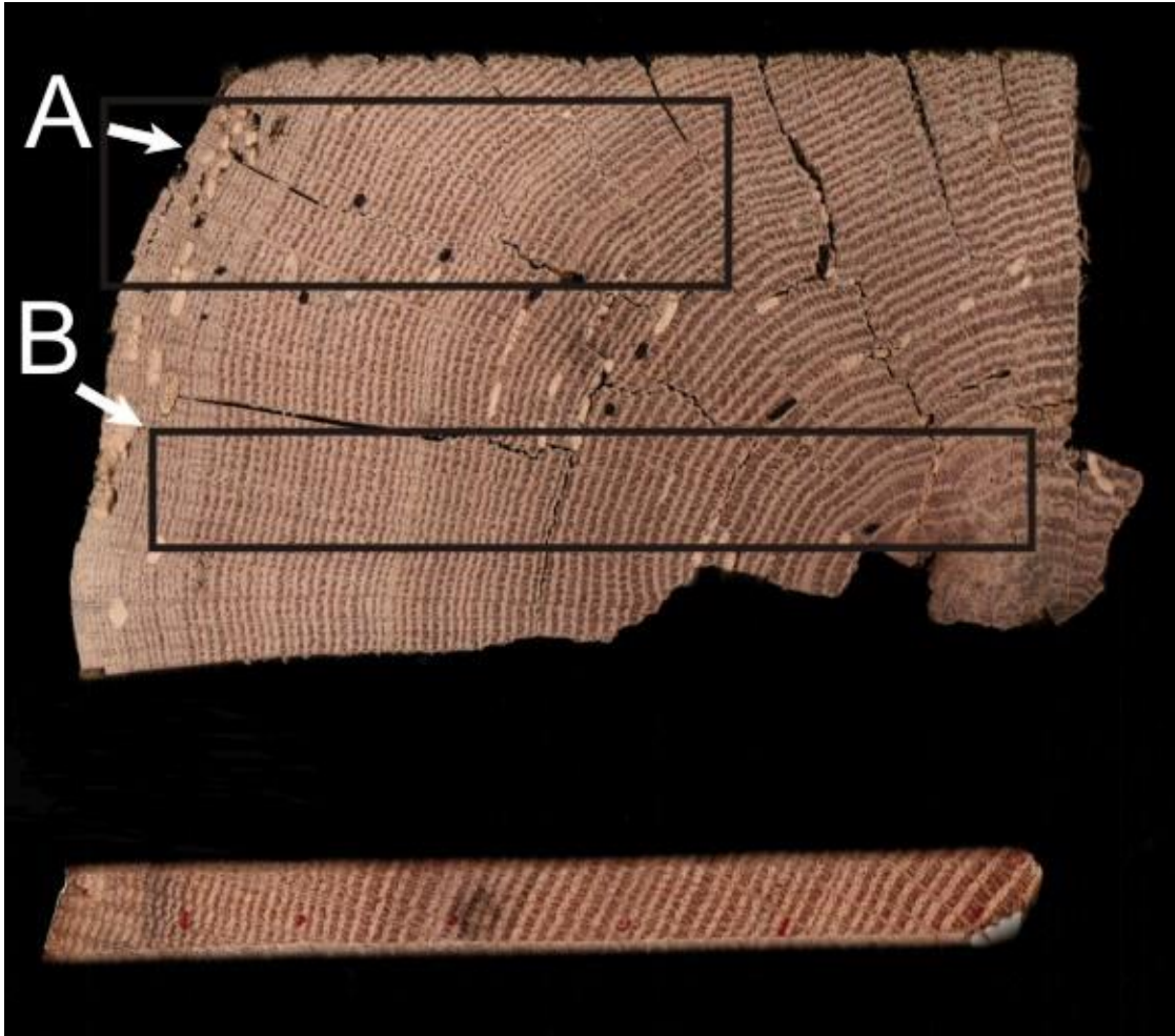
Figure 1. A cross-section of an oak timber with sapwood rings on the left-hand side (above). The boxes illustrate conversion methods resulting in A ) a precise felling date and B ) a terminus post quem or felled after date. Also pictured is a core showing complete sapwood (below).
